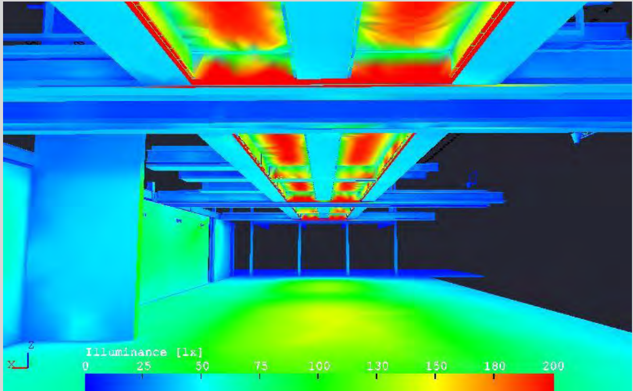
BIM Studio: IM Building Addition and Renovation Elumtools Pseudo Basement Climbers Canyon– Spring 2012
